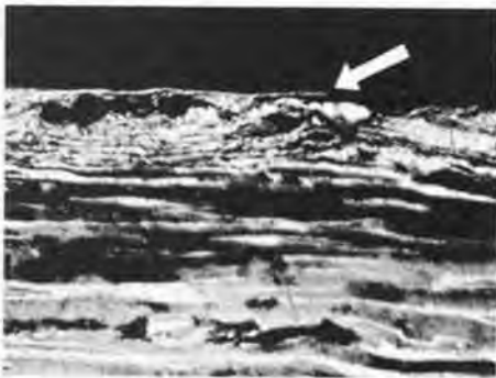
1.30 "Vicus" disk, photomicrograph of an entire section through the metal. Magnification 120X, etched by K_2Cr_2O_7 + H_2SO_4 + HCl
