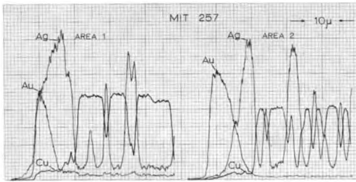
1 36 Electron microbeam probe traces of Au, Ag, and Cu across two areas of a leaf-gilded silver sheet. Area 1, single leaf layer: Ag-PET-1K; Cu-PET-10K; Au-LiF-1K. Area 2, double leaf layer: Ag-PET-1K; Cu-LiF-10K; Au-LiF-3K.
